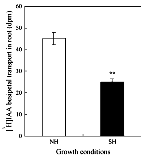
Fig. 8. The basipetal transport of [ 3 H]IAA in NH- and SH-roots. [ 3 H]IAA was applied to the apical end of 1.5 cm root segments for 1 h and the radioactivity accumulating at the basal 3 mm end of the segment was measured. Data represent averages ( \pm SE) of 40 seedlings from four independent experiments. Two asterisks represent significant differences from NH-seedlings at P < 0.05 as judged by the Student t test.
